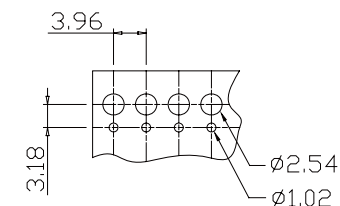
Recommended PCB Layout(B Type) (PCB TOLERANCE±0.05)
