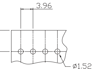
Recommended PCB Layout(A,C Type) (PCB TOLERANCE±0.05)
